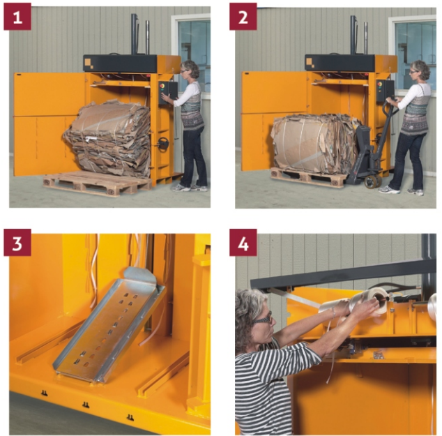
1 Compact your waste and eject the finished bale. 2 Remove and store the bale until collection. 3 An efficient and silent ejecting system ensures easy handling of the compressed bale. 4 The strap rolls are easy to replace in front of the machine.
