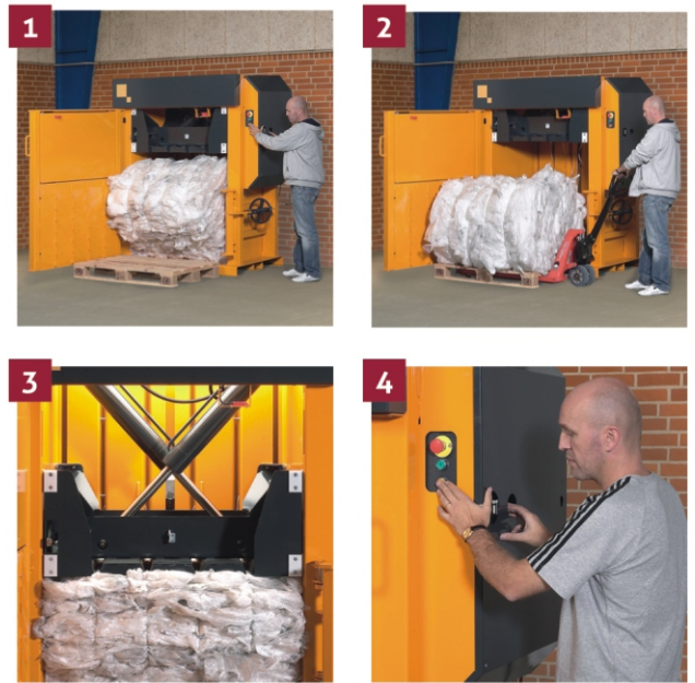
1 Compact your waste and eject the finished bale. 2 Remove and store the bale until collection. 3 The cross cylinders ensure stable compression and a low overall height. 4 The bale is ejected by a safe two-hand operation.
