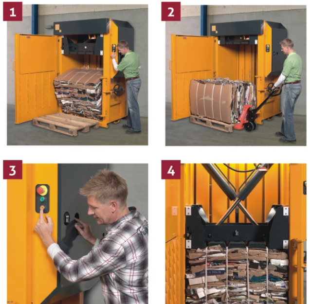
1 Compact your waste and eject the finished bale. 2 Remove and store the bale until collection. 3 The bale is ejected by a safe two-hand operation. 4 The cross cylinders ensure stable compression and a low overall height.
